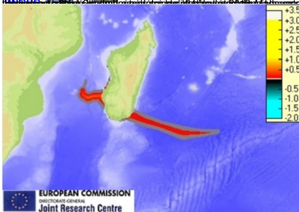
Storm surge maximum height. (Source: JRC)
